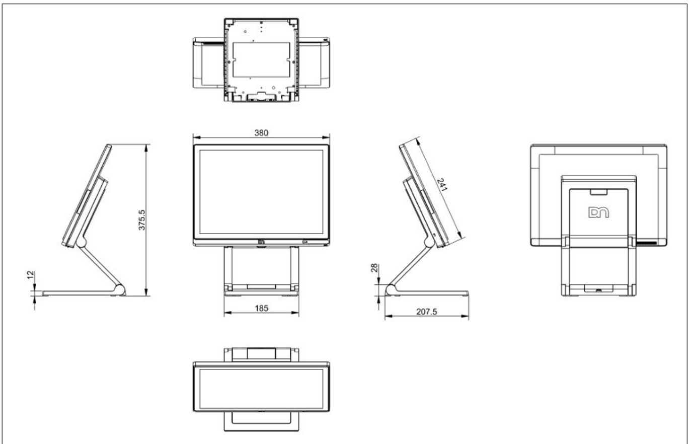
Figure 11-2: D2156 - Dimensions with stand
