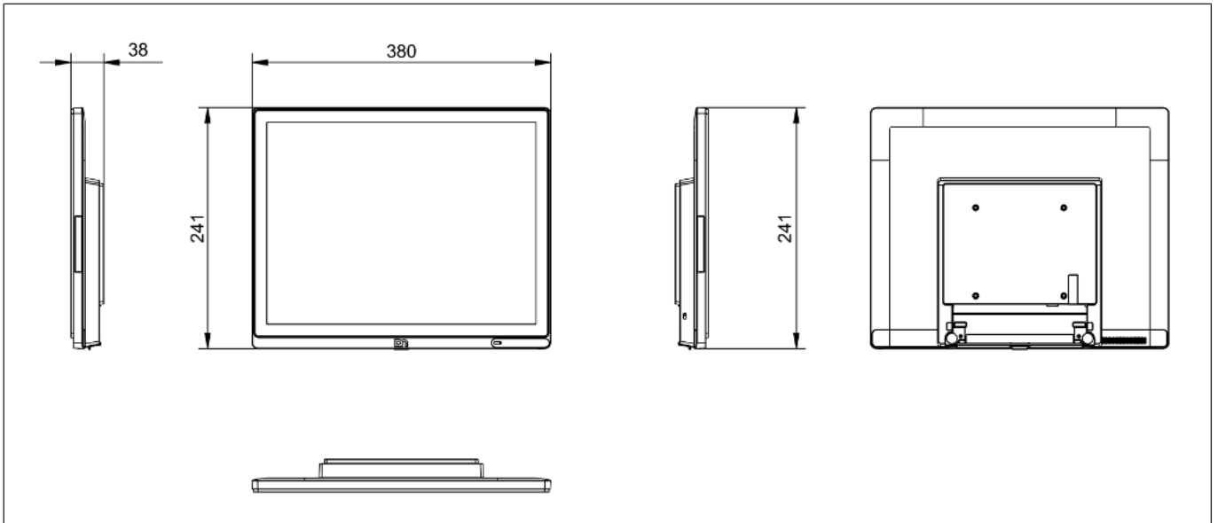
Figure 11-1: D2156 – Dimensions with wall mount
