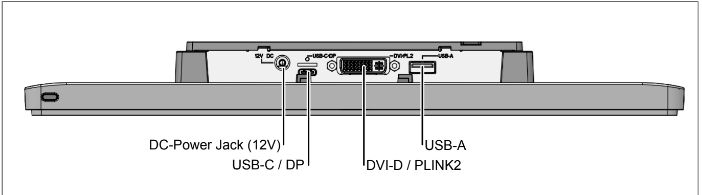
Figure 5-2: D2156 - Connector panel
