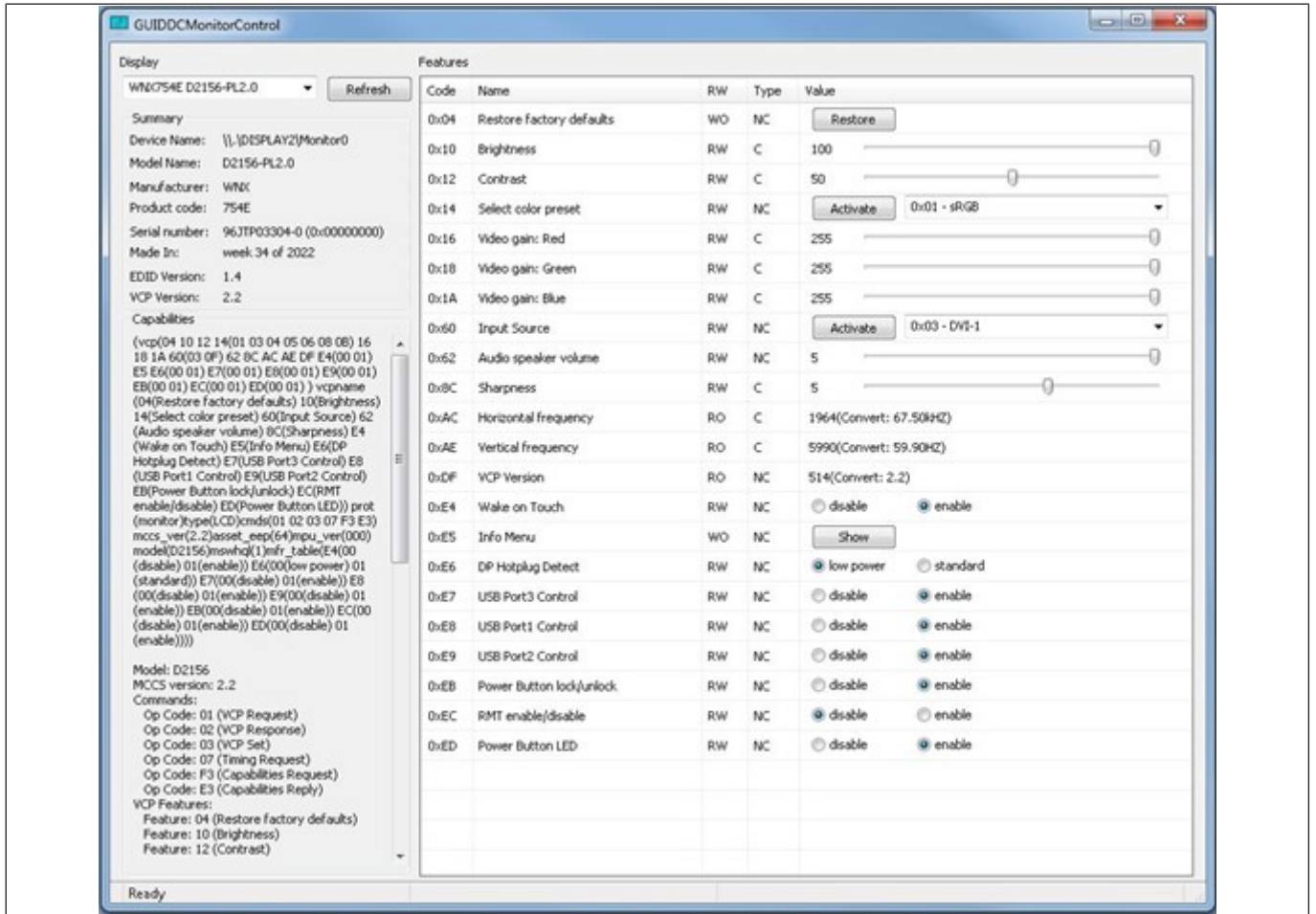
Figure 6-1: GUIDDCMonitorControl
