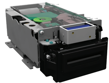
Motorized Basic Anti-Skimming Card Reader
