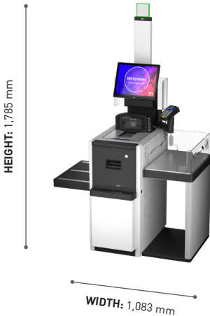
Card-only variant Height: 1,785 mm Width: 1,083 mm Depth: 718 mm
