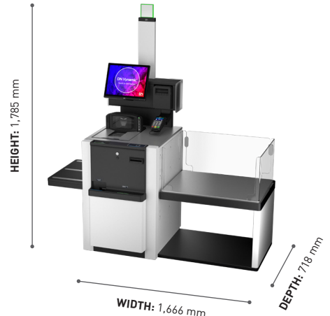
4 bagging variant Height: 1,785 mm Width: 1,666 mm Depth: 718 mm
