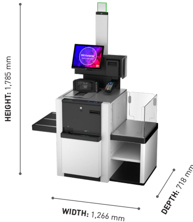
2 bagging variant Height: 1,785 mm Width: 1,266 mm Depth: 718 mm
